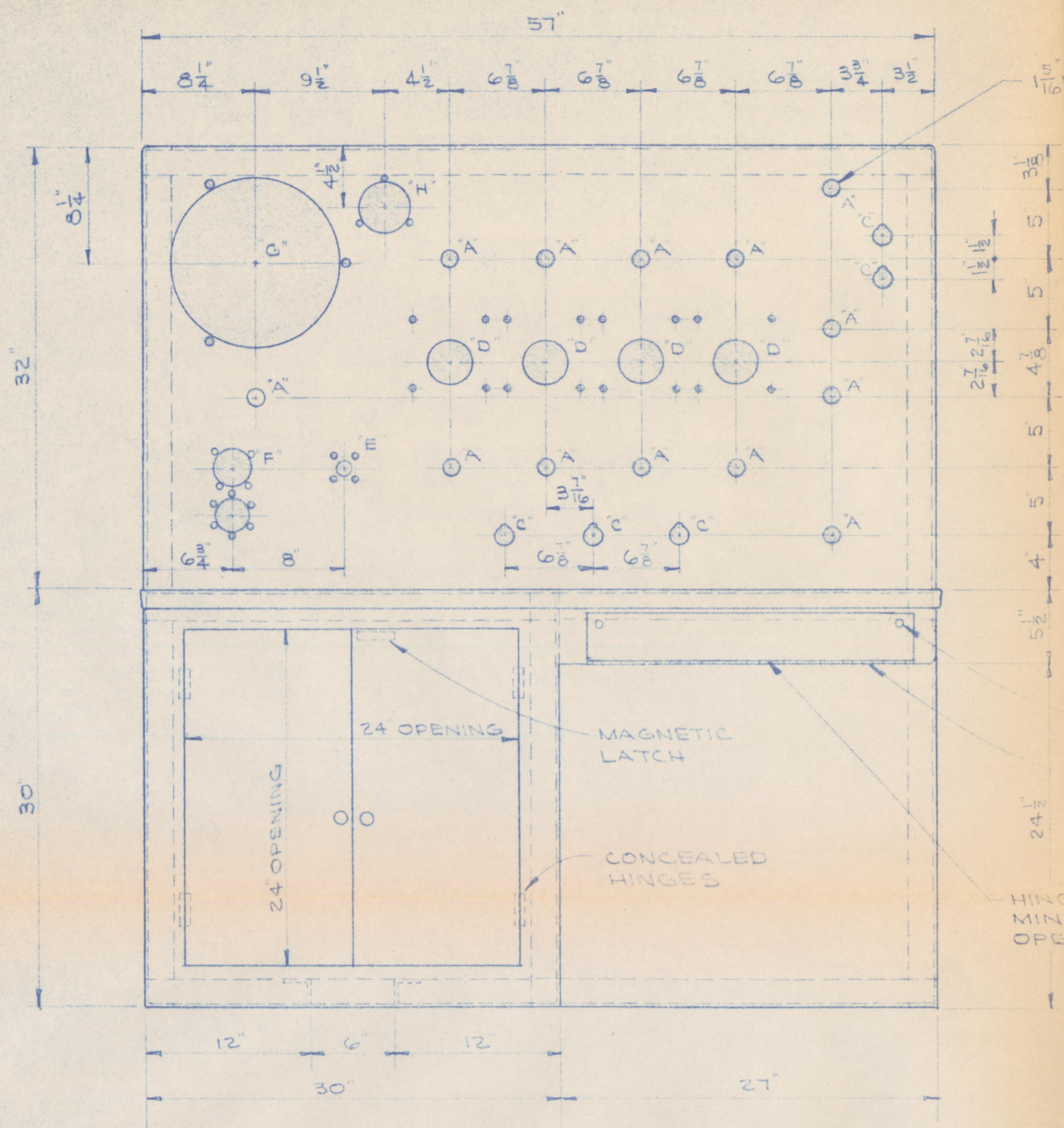
FRONT VIEW - CUTOUTS SCALE: 1 1/2" = 1" 0"
