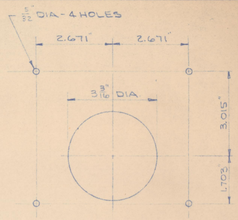
CUTOUT D SCALE: HALF SIZE 4 REQ'D.
