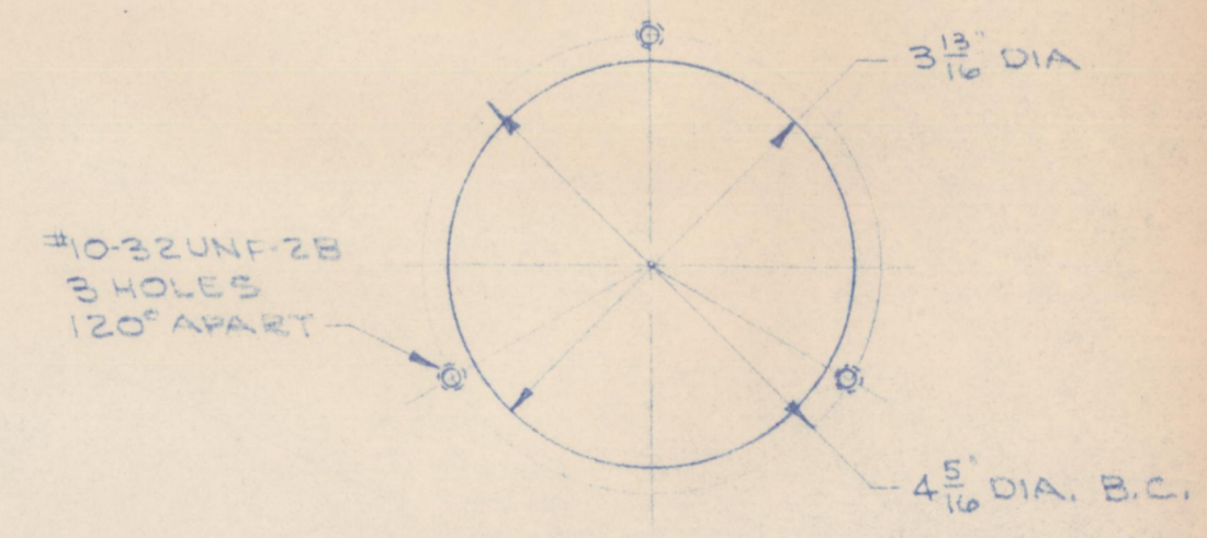
CUTOUT H SCALE: HALF SIZE 1 REQ'D.
